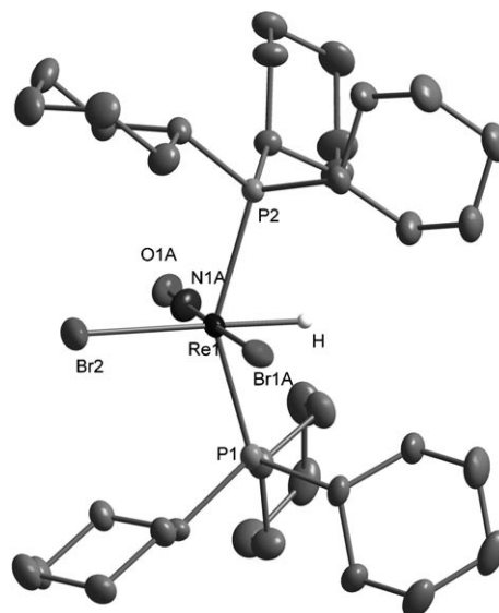
Figure 1. Molecular structure of [\text{Re}(\text{H})(\text{Br})_2(\text{NO})(\text{PCy}_3)_2] ( 3a ) at 30% probability ellipsoids (selected hydrogen atoms and the trans -NO/Br positional disorder have been omitted for clarity). Selected bond lengths [Å]: P1–Re1 2.4709(7), P2–Re1 2.4732(8), Br1A–Re1 2.5213(6), N1A–O1A 1.229(6), Br2–Re1 2.5809(4). Selected bond angles [°]: P1–Re1–P2 147.94(2), O1A–N1A–Re1 179.0(4), N1A–Re1–Br1A 178.87(16), P1–Re1–H 74.6(11), P2–Re1–H 73.4(11), P1–Re1–Br2 106.486(18), P2–Re1–Br2 105.45(2), P1–Re1–Br1A 90.00(2), Br2–Re1–H 172.0(11).
