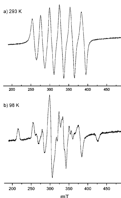
Figure 2. a) X-band EPR spectra of a solution of 3b in toluene at 293 K (top). b) Low-temperature glass spectrum of 3b at 98 K (bottom).
