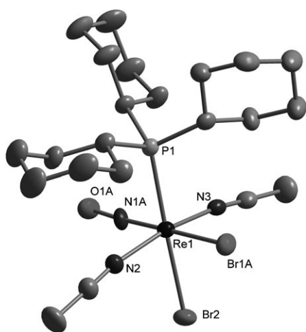
Figure 5. Molecular structure of [Re(Br) 2 (NO)(MeCN) 2 (PCy 3 )] ( 8a ) with 30% probability displacement ellipsoids. The trans -NO/Br disorder and all hydrogen atoms have been omitted for clarity. Selected bond lengths [Å]: P1–Re1 2.4311(7), N1A–Re1 1.831(7), N2–Re1 2.060(2), N3–Re1 2.054(2), N1A–O1A 1.226(8). Selected bond angles [°]: P1–Re1–Br2 178.461(18), N1A–Re1–Br1A 178.7(3), N3–Re1–N2 168.66(9), O1A–N1A–Re1 173.5(10), Br1A–Re1–P1 92.28(5).
