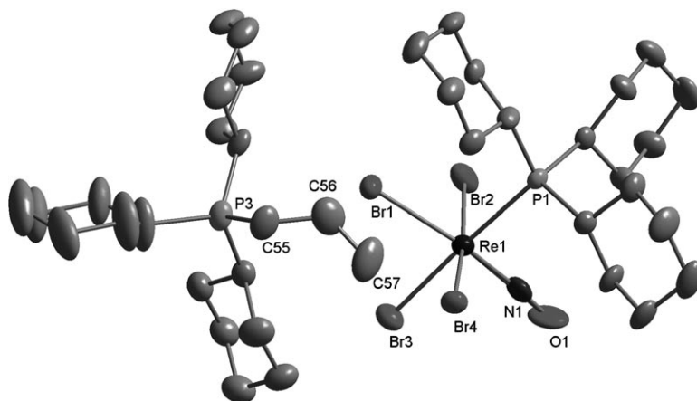
Figure 4. Molecular structure of [\text{Cy}_3\text{PCH}_2\text{CH}=\text{CH}_2][\text{Re}(\text{Br})_4(\text{NO})(\text{PCy}_3)] ( 6a ) with 20% probability displacement ellipsoids. Two of the four independent molecules are shown. All hydrogen atoms have been omitted for clarity. Selected bond lengths [Å]: Re1–N1 1.793(11), Re1–Br2 2.5147(11), Re1–Br4 2.5215(11), Re1–P1 2.546(3), Re1–Br3 2.5618(11), Re1–Br1 2.5718(11), N1–O1 1.046(12). Selected bond angles [ ^\circ ]: N1–Re1–Br1 169.8(3) , P1–Re1–Br3 176.32(6) , N1–Re1–Br2 89.3(3) , N1–Re1–Br4 97.8(3) , O1–N1–Re1 173.6(11) .
