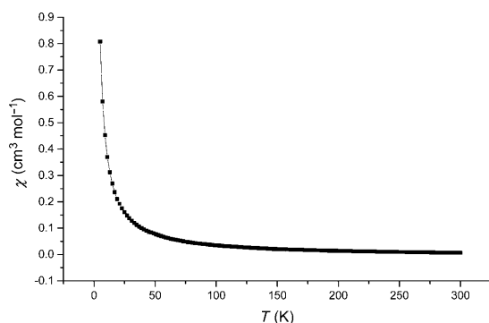
Figure 3. Temperature-dependent magnetic susceptibility data of 3a recorded in the range of 5–300 K.
